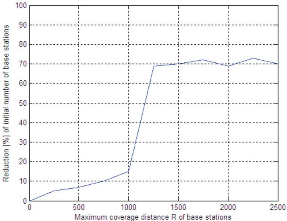
Figure 9: Reduction [%] of the initial number of BSs as a function of the maximum coverage distance R_{BS} (emitted power) of BSs to be installed.
