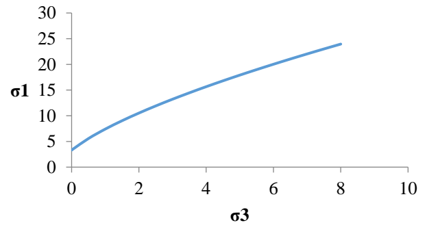
Figure 4. Graph shows the Sheorey - Failure criterion
