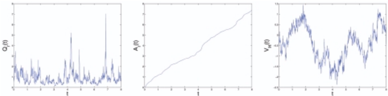
Figure 3. Sample of a realization of (left) Q_r(t) , (middle) A(t) and (right) V_H(t) .
