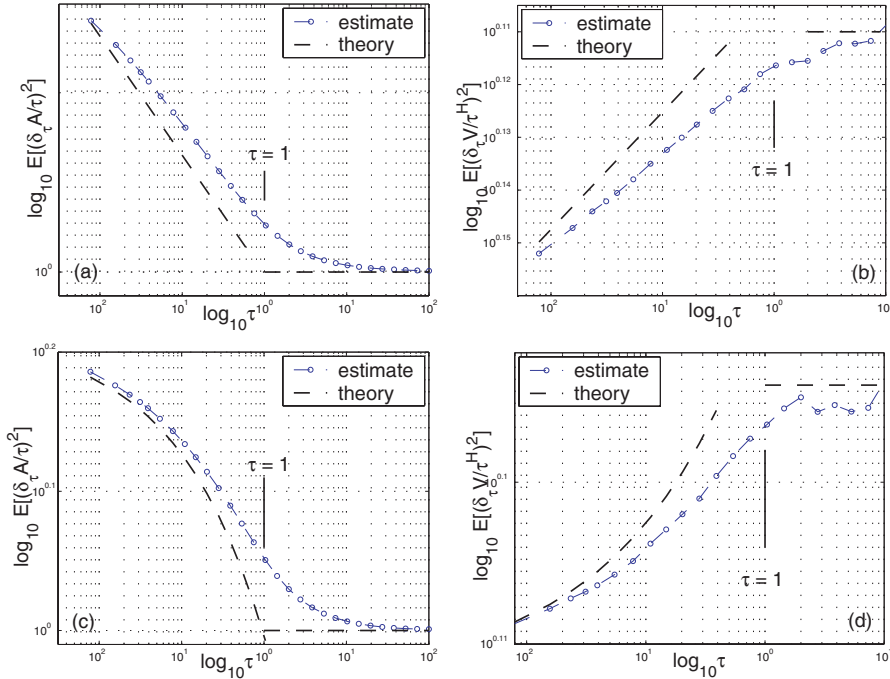
Figure 6. A power law scaling cascade: (a) \ln \mathbb{E}[(\delta_\tau A/\tau)^2] compared to c\varphi(2) \ln \tau + Cte . (b) \ln \mathbb{E}[(\delta_\tau V/\tau^H)^2] compared to c\varphi(2H) \ln \tau + Cte . A warped cascade deviates from power laws: (c) \ln \mathbb{E}[(\delta_\tau A/\tau)^2] compared to -\varphi(2)m(C_\tau) ; (d) \ln \mathbb{E}[(\delta_\tau V/\tau^H)^2] compared to -\varphi(2H)m(C_\tau) . Power law scaling is associated to straight lines in log-log diagrams.
