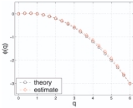
Figure 7. Estimated exponents \varphi(q) correspond to prescribed theoretical ones.
