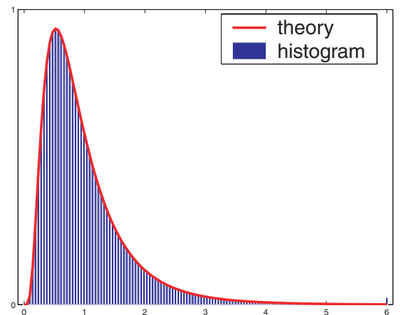
Figure 4. Histogram of Q_r compared to its theoretical log-Normal probability density function: the agreement is perfect.
