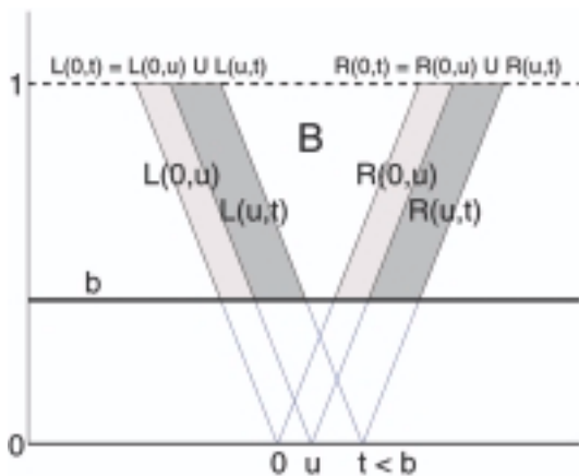
Figure 11. Definition of \mathcal{L} , \mathcal{B} and \mathcal{R} .
