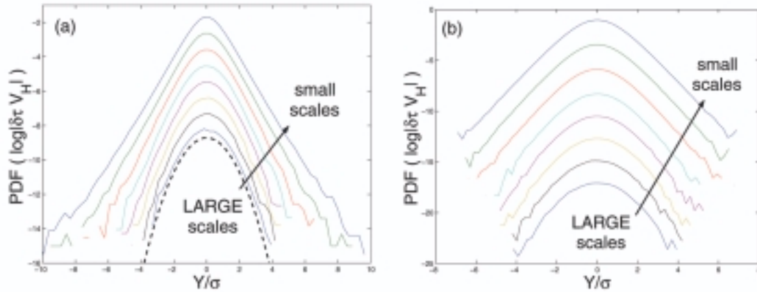
Figure 9. Evolution of probability density functions of the increments \delta_\tau V_H from Gaussian at large scales to non Gaussian at smaller scales, respectively for (a) a power law scaling cascade and (b) a warped cascade.
