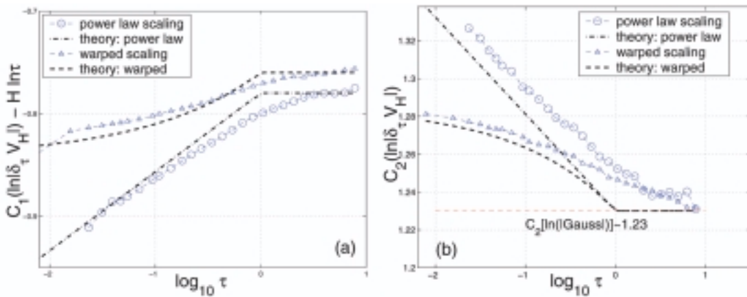
Figure 10. Cumulants of the log of increments of V_H from a warped cascade deviates from power laws: (a) C_1 - H \ln \tau compared to -H\phi'(0)m(C_\tau) ; (b) C_2 compared to -H^2\phi''(0)m(C_\tau) .
