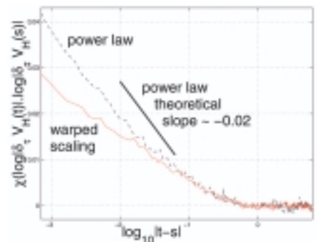
Figure 8. Autocorrelation of the log of increments of V_H from a warped cascade deviates from logarithmic behavior.
