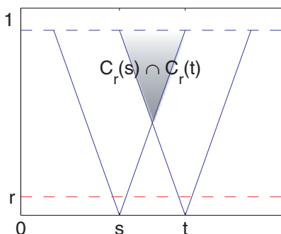
Figure 2. Dependence between Q_r(t) and Q_r(s) , in particular their correlation, stems entirely from the contribution of the intersection of two cones \mathcal{C}_r(t) and \mathcal{C}_r(s) .
