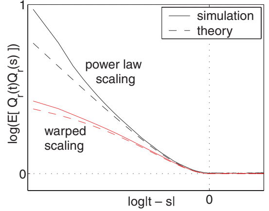
Figure 5. Theoretical and estimated autocorrelation functions of Q_r respectively in a power law scaling case ( dm(t,r) = dt dr/r^2 ) and a warped scaling case ( dm(t,r) = dt dr/r^{2+\beta} ): it is sensitive to a departure from the reference power law behavior in a controlled manner.
