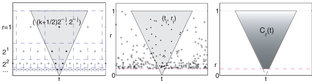
Figure 1. Comparison between the "time-scale" construction of multiplicative cascades. (left) Binomial cascade, (center) Compound Poisson Cascade, (right) Infinitely Divisible Cascade. The grey region indicates the cone containing multipliers that determine the value of the density at time t .
