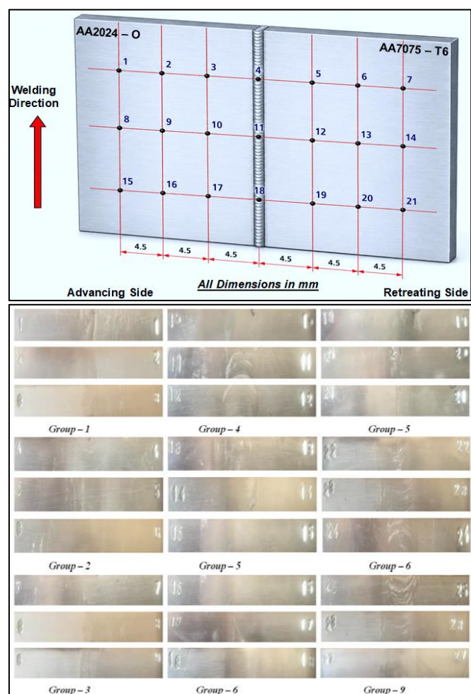
Figure 1. The locations where the welded pieces' microstructure was investigated
