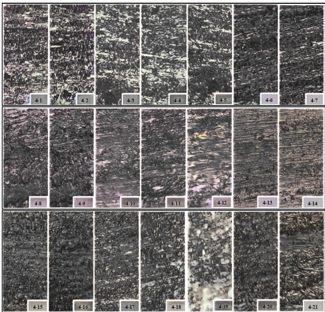
Figure 5. Surface microstructure on the fourth model (Group 4) in different locations
