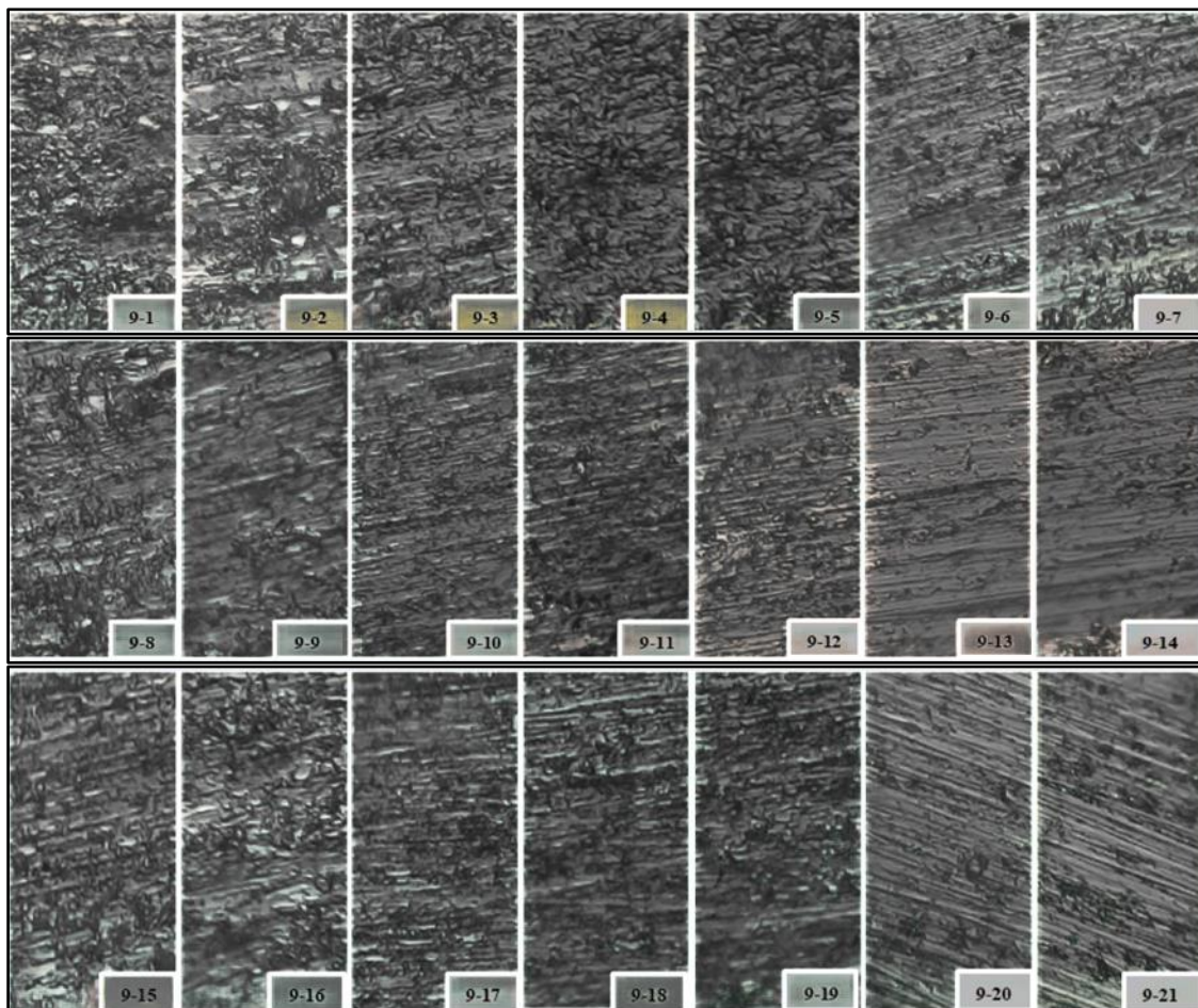
Figure 10. Surface microstructure on the third model (Group 9) in different locations
