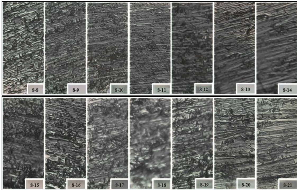
Figure 9. Surface microstructure on the third model (Group 8) in different locations
