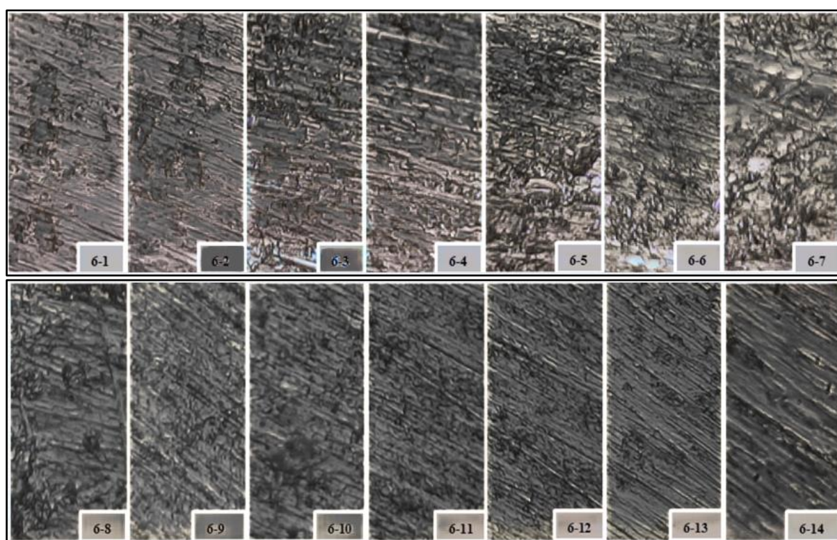
Figure 6. Surface microstructure on the third model (Group 5) in different locations
