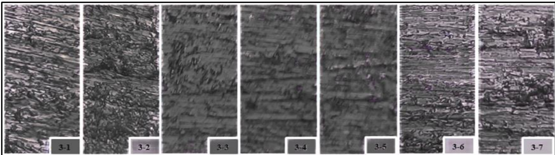
Figure 3. Surface microstructure on the second model (Group 2) in different locations
