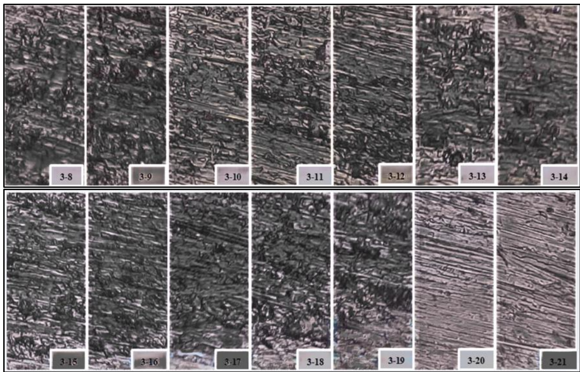
Figure 4. Surface microstructure on the third model (Group 3) in different locations
