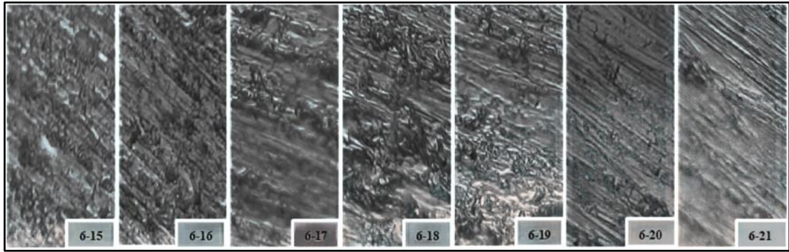
Figure 7. Surface microstructure on the third model (Group 6) in different locations
