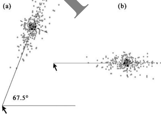
Figure 8. (a) Integrating the bivariate normal distribution rotated by 67.5^\circ over the region defined by a rectangle. (b) Integrating the nonrotated bivariate normal distribution over the region defined by a rectangle rotated by -67.5^\circ
