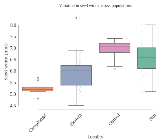
Figure 3. Variation in seed width (mm) among rice bean ( V. umbellata ) populations from Camplong 2, Ekateta, Oinlasi, and Sillu on Timor Island, Indonesia
