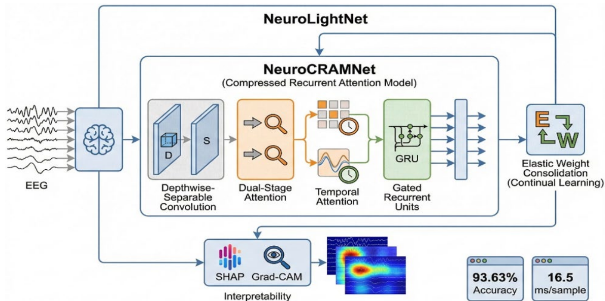
Figure 1. Overall architecture diagram of the proposed model
