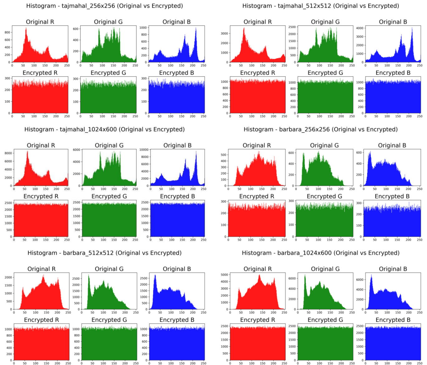
Figure 4. Histogram analysis
