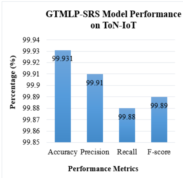
Figure 5. GTMLP-SRS performance on Telemetry over Network–Internet of Things (ToN-IoT) dataset
