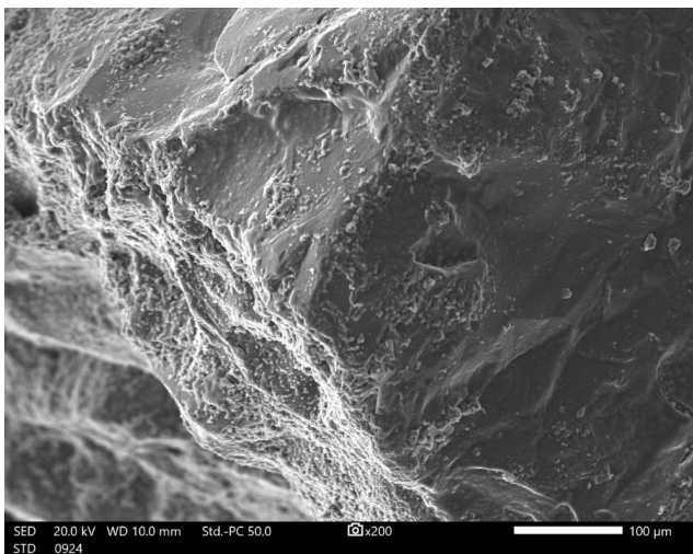
Figure 7. SEM image of quartz material after second nanoparticle coating showing increased surface coverage
