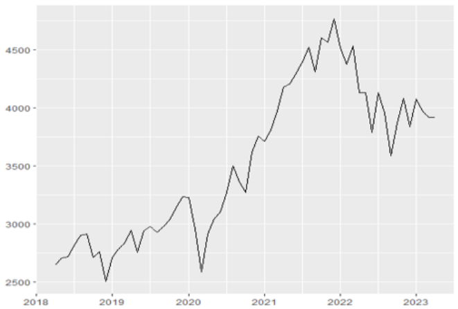
Figure 3. S&P price using ARIMA model till March 2023
