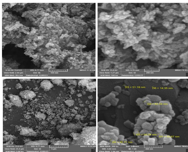
Figure 5. FESEM illustration of nano-hydroxyapatite (Nano-HAP)
