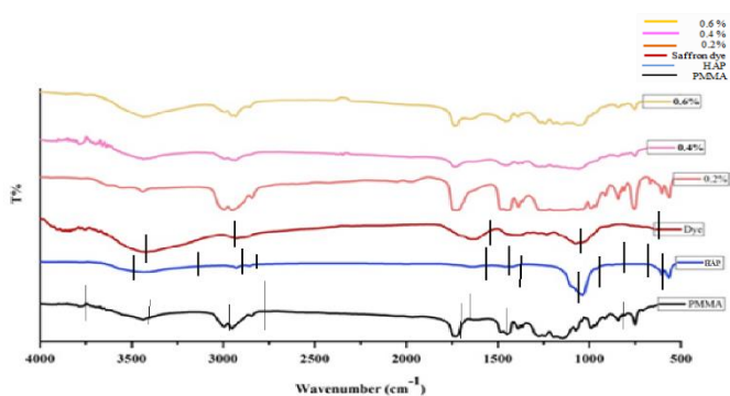
Figure 6. FTIR spectroscopy illustration of composites (PMMA/Nano-HAP+saffron dye)
