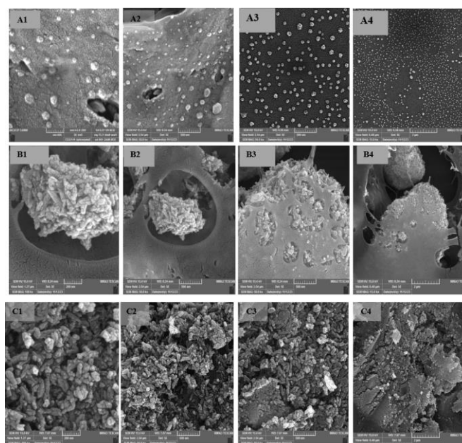
Figure 7. SEM images of Poly (methyl methacrylate) cross-section of unmodified (PMMA pure) (A1–A4), modified PMMA(B1-B4) (PMMA/Nano-HAP (0.2g) +saffron dye) and modified PMMA(C1-C4) (PMMA/Nano-HAP (0.6g) +saffron dye)
