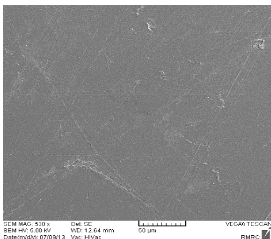
Figure 3. SEM image of virgin (pure) PP at 210°C
