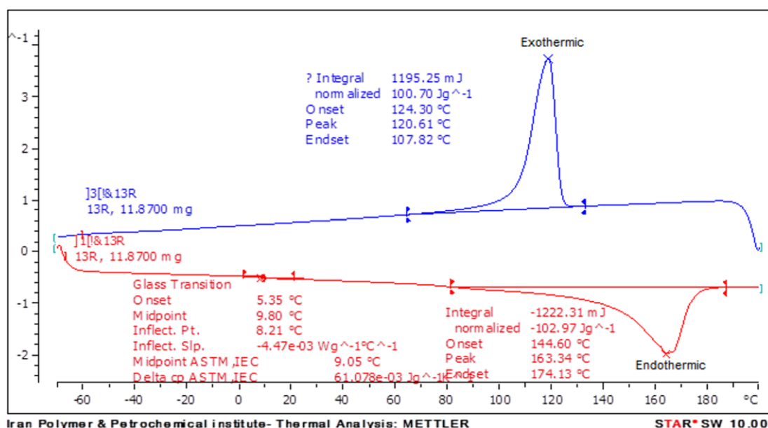
Figure 4. DSC test results for virgin PP
