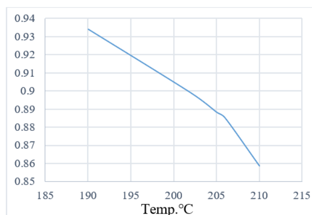
Figure 7. Density behavior with processing temperature change
