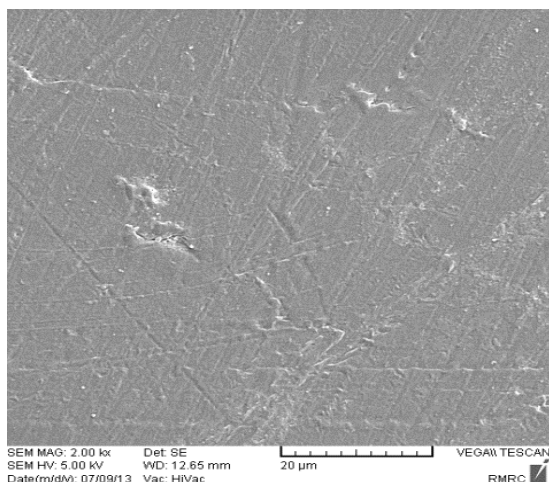
Figure 2. SEM image of virgin (pure) PP + recycled PP at 210°C
